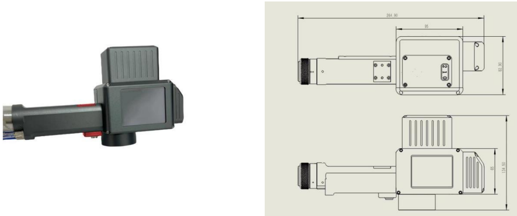
Figure 2.3 GY-QBDXYP1000 cleaning head structure and main dimensions (dust suction port and bracket are optional accessories)
