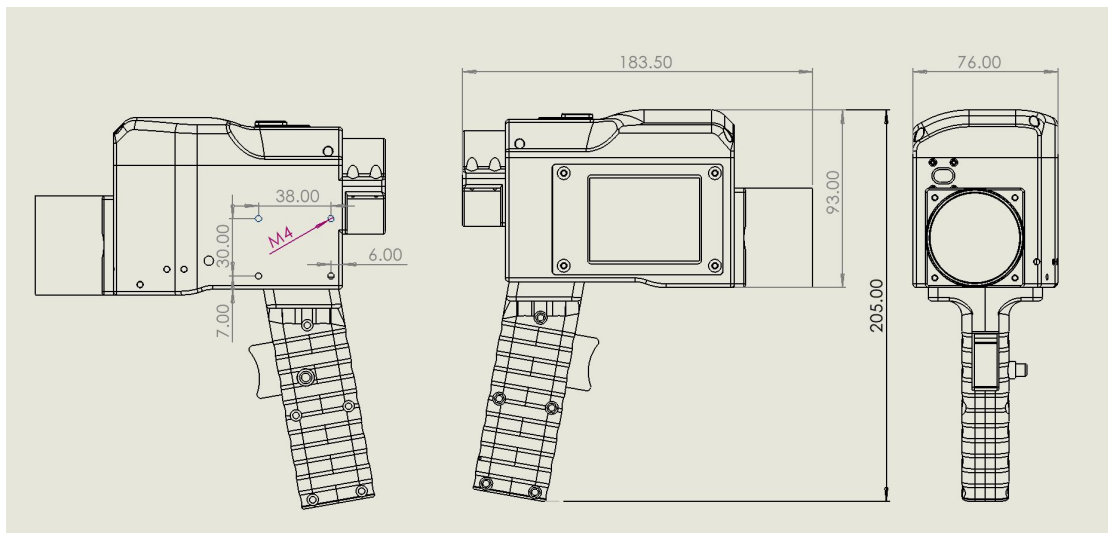
Figure 2.3 GY-QBFXYP500 cleaning head structure and main dimensions (dust suction port and bracket are optional accessories)
